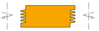
Profile 2 with staggered shoulder cutters
