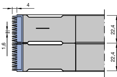
Minifinger joint cutter ZL 4 mm, TG 1.6 mm
